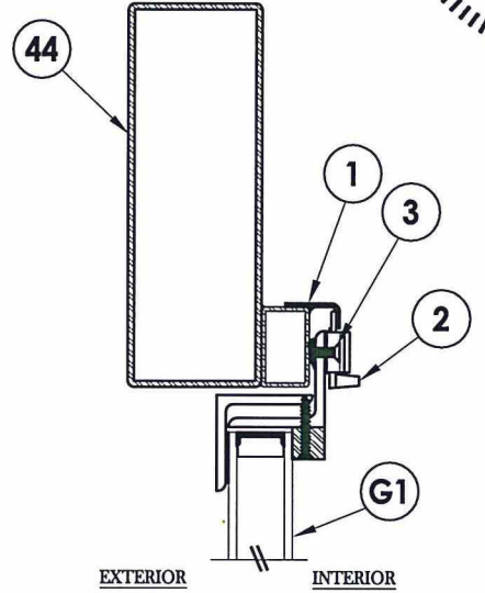
2 VERTICAL CROSS SECTION
