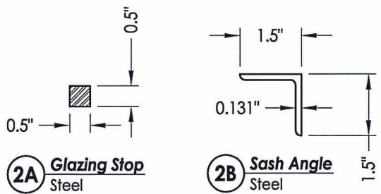
G1 GLAZING DETAIL Operable Door/Sidelite
